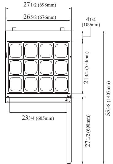
PLAN VIEW
